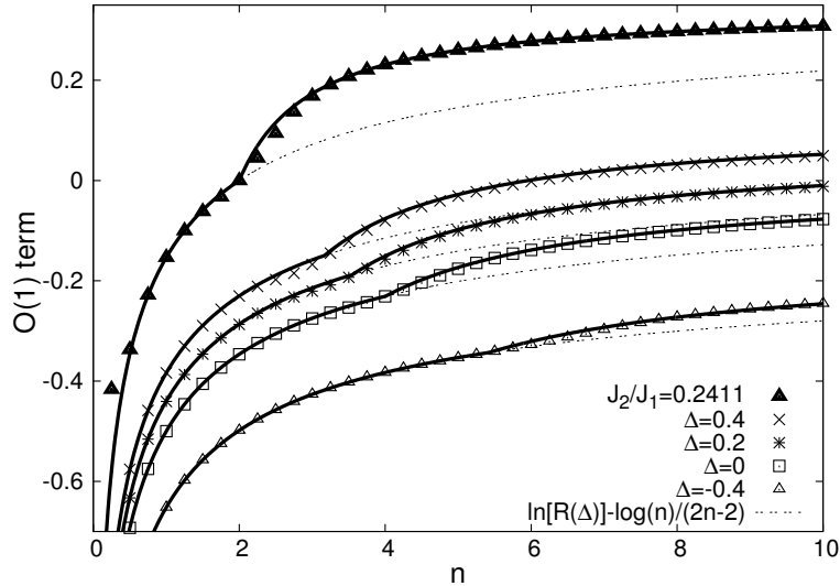
Figure 2.1: Constant term in the SRE of periodic XXZ and J_1 - J_2 chains for different values of \Delta and at the critical point J_2/J_1 = 0.2411 . Each point comes from fitting the data for L = 20, 22, 24, 26 and 28 to aL + b + c/L + d/L^2 . Fat lines: theoretical prediction (Eq. 1.52). The prediction for n < n_c is also plotted above n_c (dashed lines) for comparison. The J_1 - J_2 chain ( SU(2) symmetric, but with second neighbor interaction) lies at the transition point between a TL liquid phase and a dimerized one. It has R = \sqrt{2} , as the XXZ chain at \Delta = 1 , but no logarithmic corrections (hence smaller finite-size effects). Taken from [5].
