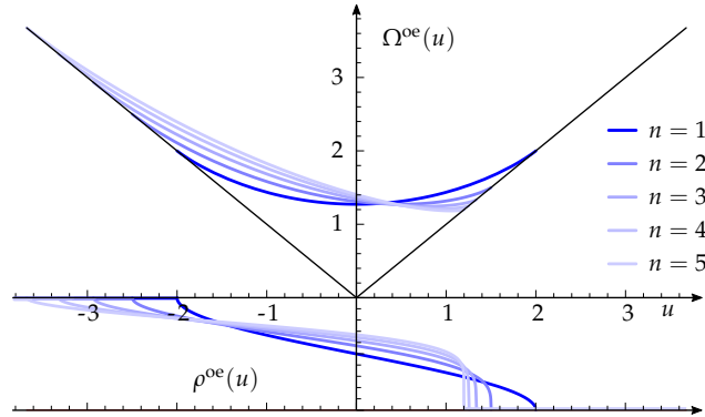
Figure 2: Limit shape and density profile of \mathbb{P}_{n,\theta}^{oe} -distributed random partitions.
