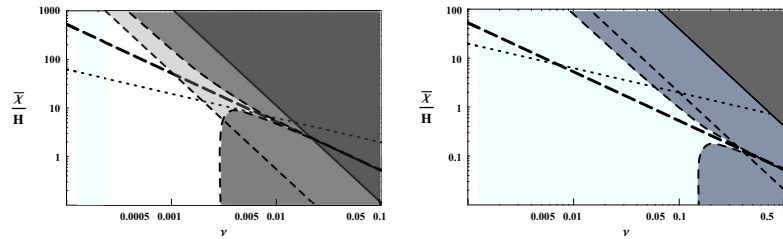
Figure 3. Exclusion diagrams for parameters \nu and \bar{\chi} for \theta = \pi/4 (left panel) and for \theta = 0.1 (right panel). The gray areas are the exclusion zones, dark gray corresponding to the constraints derived from WMAP and medium and light gray for the constraints expected from Planck. The straight line boundaries correspond to bispectrum observations (of slope -2 ), the other case to the trispectrum. The long dashed is the location where the terms contributing to the trispectrum cancel. We adopted the results of [41] on the upperbounds the Planck mission is expected to provide, f_{\text{NL}} = 5 and \tau_{\text{NL}} = 560 . The dotted lines are the locations where \bar{\chi} is equal to its expected 1\text{-}\sigma fluctuation.
