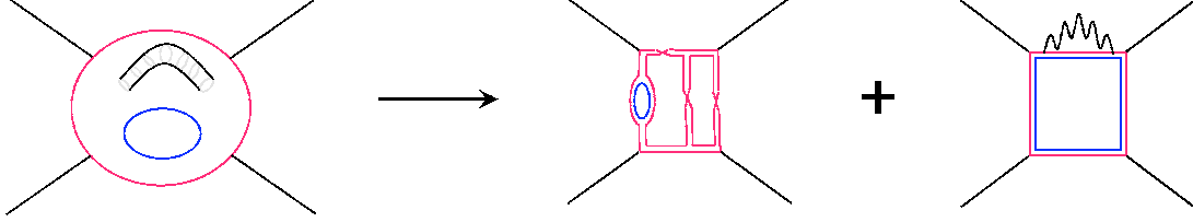
Fig. 2: A world-sheet with one handle and two boundaries that contributes to the single-trace term at the same order as the four-boundary amplitude of figure 1. The figure illustrates examples of field theory diagrams that arise from the short-handle and long-handle boundaries of moduli space in the low energy limit.
