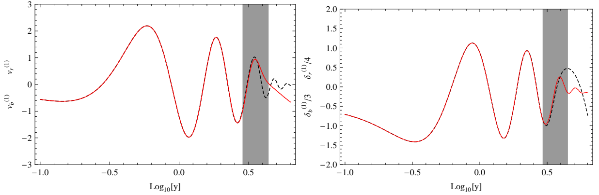
FIG. 8: Left: Comparison of the baryons and photons velocity perturbation at first order for k = 10k_{\text{eq}} . It shows that v_r^{(1)} = v_b^{(1)} with a good approximation until decoupling. Right: Comparison of \frac{1}{4}\delta_r^{(1)} and \frac{1}{3}\delta_b^{(1)} . It can be seen that the adiabaticity condition holds until recombination, hence justifying the approximation of § III.
