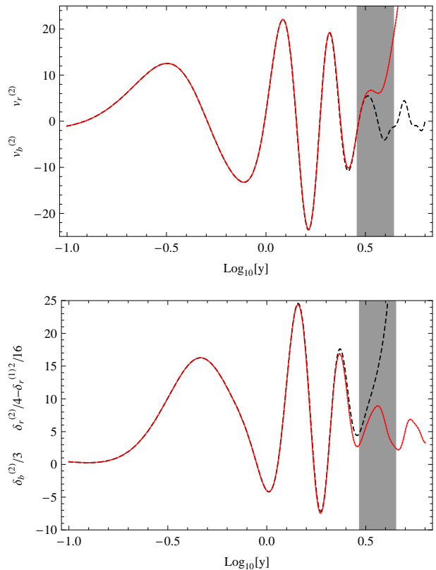
FIG. 2: Top: Comparison of the baryons and photons velocity perturbation at order 2 for k_1 = k_2 = 10k_{\text{eq}} and \mathbf{k}_1 \cdot \mathbf{k}_2 = 0 . It shows that v_r^{(2)} = v_b^{(2)} with a good approximation until decoupling. Bottom: l.h.s and r.h.s of Eq. (45) for the adiabaticity condition at order 2. It can be seen that this adiabaticity condition holds until recombination, hence justifying the approximation of § III.
