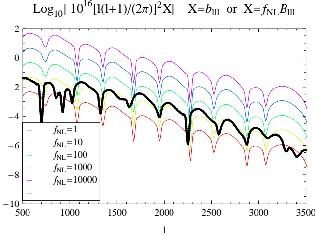
FIG. 6: Black: the bispectrum for the equilateral configuration computed in the flat sky limit. The thin colored lines represents the bispectrum that would be obtained by assuming a constant initial f_{\text{NL}}^{\Phi} and a linear transfer function, that is neglecting the non-linear dynamics. From bottom to top we have plotted f_{\text{NL}}^{\Phi} = 1, 10, 100, 1000, 10000 .
