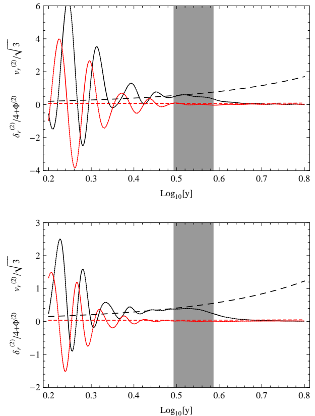
FIG. 5: Behavior of \Theta_{SW}^{(2)} (black) and kv_r^{(2)}/\sqrt{3} (red). The numerical integration is depicted with solid lines while the analytical estimates is plotted in dashed lines. From top to bottom, we have k_1 = k_2 = 30 k_{\text{eq}} , and k_1 = k_2 = 40 k_{\text{eq}} . The vertical grey zone represents the “surface” of last scattering.
