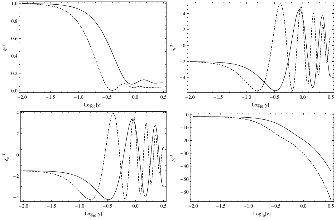
FIG. 7: From top to bottom, left to right: evolution of the Bardeen potential, \Phi , and the density contrast \delta for respectively radiation, baryons and cold dark matter. The solid line corresponds to k = 10k_{\text{eq}} and the dashed line corresponds to k = 20k_{\text{eq}} .
