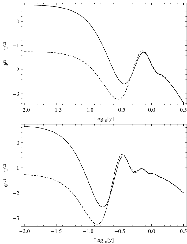
FIG. 1: Evolution of the two second order gravitational potentials, \phi^{(2)}(\mathbf{k}_1, \mathbf{k}_2) and \psi^{(2)}(\mathbf{k}_1, \mathbf{k}_2) for k_1 = k_2 = 10k_{\text{eq}} (top panel) or k_1 = k_2 = 20k_{\text{eq}} (bottom panel) and \mathbf{k}_1 \cdot \mathbf{k}_2 = 0 .
