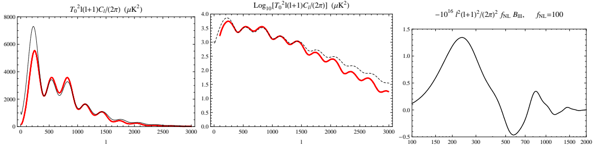
FIG. 9: Left: in solid red line, the angular power spectrum using our code and the flat sky approximation (which does not include the late ISW). The black dashed line represents the spectrum obtained using CAMB, which also takes into account the late ISW, but no reionisation. Middle: The precision on small scale depends highly on the computation of the visibility function. On small scales, our transfer function is approximately 30% smaller than the one predicted by CAMB and is thus a good approximation. Right: the bispectrum obtained from a primordial constant f_{NL} = 100 evolved linearly.
