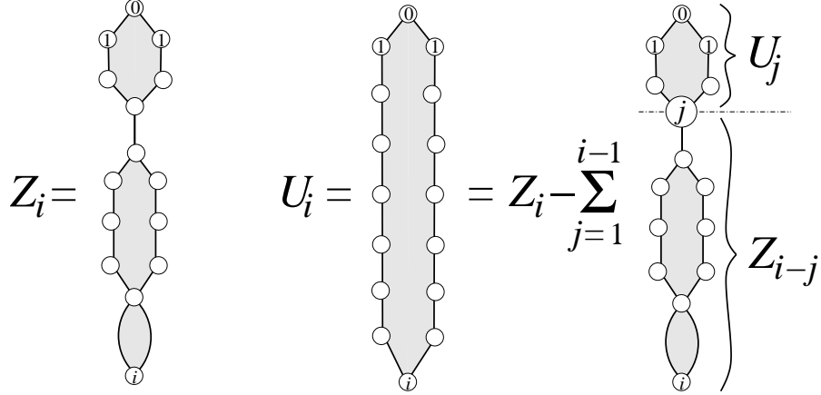
Fig. 9: A schematic picture of the configurations of quadrangulations with a geodesic boundary of length 2i as counted by Z_i (generic case) or U_i (case with no pinch point), and of their relation (2.5).
