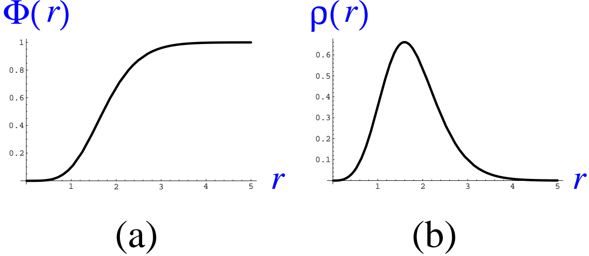
Fig. 16: The distribution function \Phi(r) measuring the probability that a vertex be at a rescaled distance less than r in the scaling limit of large quadrangulation. Its derivative \rho(r) is the density of vertices at rescaled distance r .
