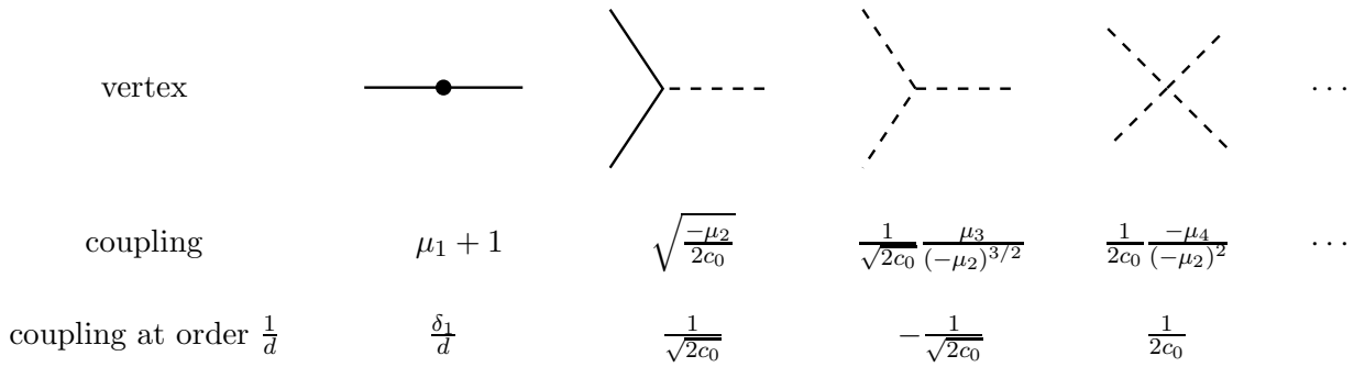
FIG. 7 The vertices contributing to -V^{\text{inst}}(r) and their couplings in the large- d -reorganized perturbative expansion.
