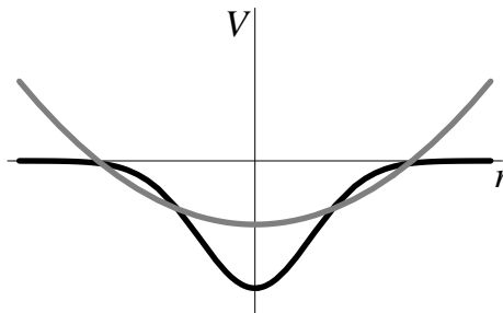
FIG. 4 The variational instanton (black) and its approximation by a harmonic potential (grey) (here for D = 1 , d = 4 ). Note that the curvature of V(r) is the quadratic term before normal-ordering, whereas in the variational approximation the quadratic term after normal-ordering appears.
