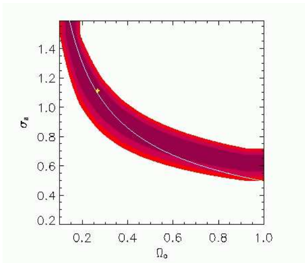
Fig. 2. The \Omega_0 - \sigma_8 constraint derived from combined cosmic shear surveys. The three grey areas define the 1, 2 and 3- \sigma limits. The cross indicates the position of the best fit at \Omega_0 = 0.26 and \sigma_8 = 1.1 . The solid line shows the local cluster abundance best fit ([11]). The latter and the cosmic shear constraints have similar shape and match very well.
