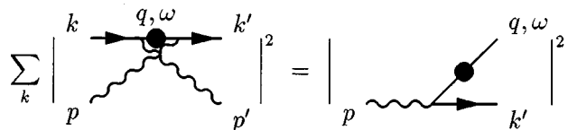
FIG. 9. Left: Leading diagram for Compton scattering in the limit of soft exchanged momenta. Right: Emission of a soft virtual positron (or absorption of a soft electron) by a hard photon, corresponding to the process on the left.
