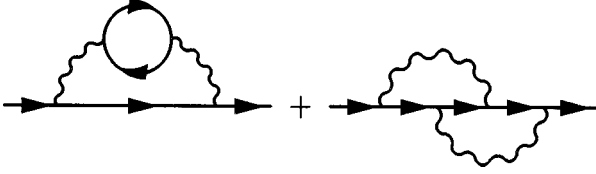
FIG. 4. Two-loop self-energy diagrams corresponding to the scattering processes depicted in Fig. 3. The diagram on the left gives the direct and exchange contribution while the diagram on the right is the interference term.
