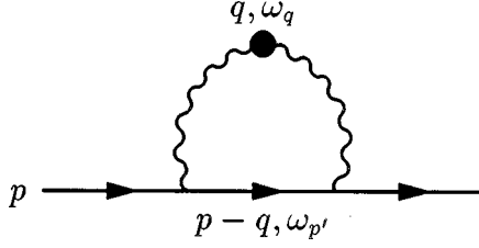
FIG. 17. One-loop resummed diagram contributing to the electron or quark damping rate.
