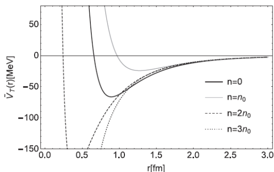
FIG. 2. \tilde{V}_T(r) = V_T(r)(\tau_1\tau_2S_{12})^{-1} at various densities n [3]. Note that the \rho -tensor force is suppressed almost completely at n \gtrsim 2n_0 .
