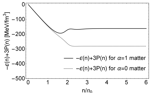
FIG. 4. \langle \theta_\mu^\mu \rangle in V_{lowk} RG reproduced from [3].
