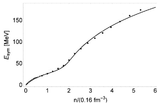
FIG. 3. The symmetry energy E_{sym} in V_{lowk} RG reproduced from [3].
