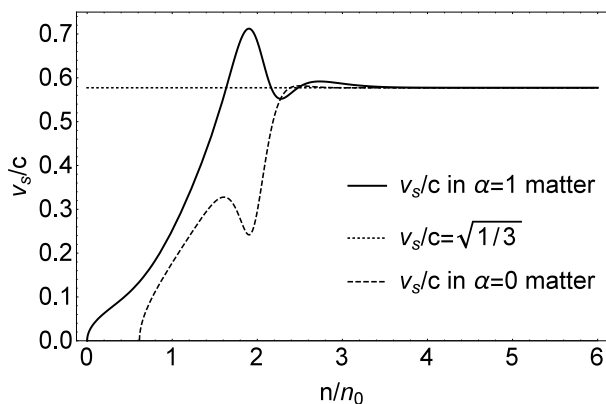
FIG. 5. Sound velocity calculated in V_{lowk} RG.
