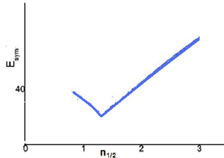
FIG. 1. Schematic cusp structure for E_{sym} reproduced from [5]. The energy and density scales are arbitrary. What is relevant is the generic cusp structure which depends only on topology, hence only on the pion field.
