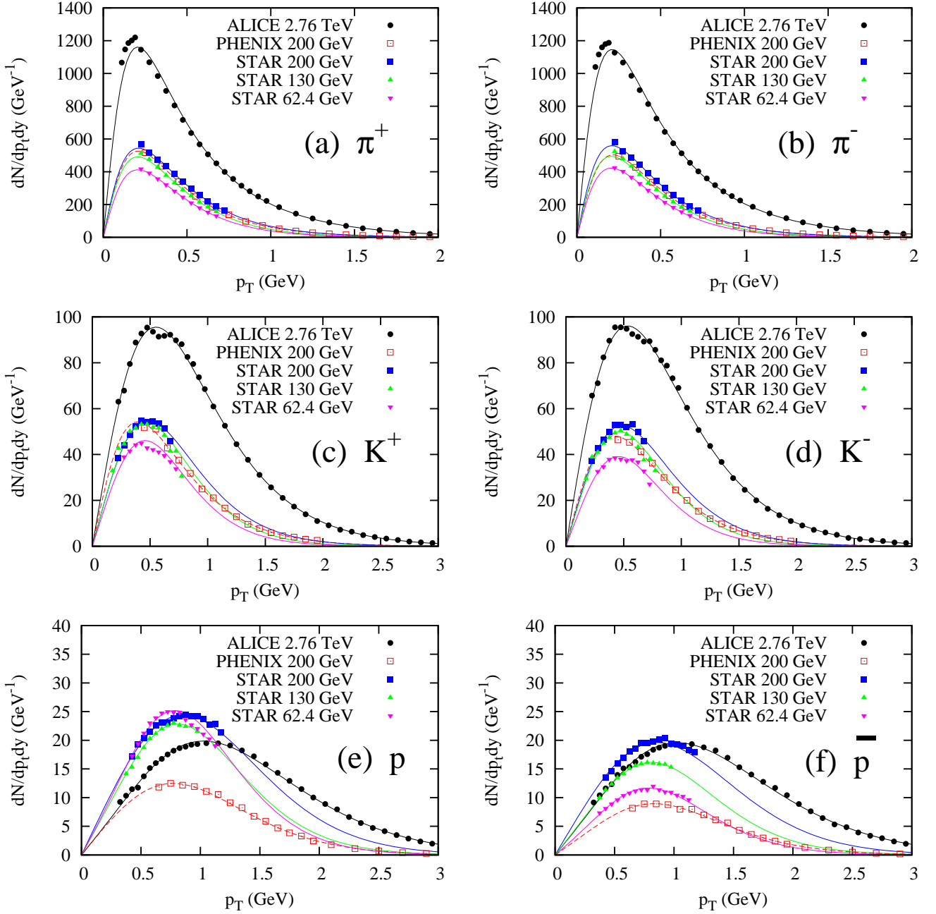
FIG. 8. (Color online) Transverse momentum distributions of identified particles in Pb+Pb collisions at the LHC and Au+Au collisions at RHIC. The centrality range is 0-5% for all sets of data except 130 GeV data which are 0-6%. Symbols are data from ALICE [73], PHENIX [72] and STAR [71, 74]. Solid lines are blast-wave fits (see text). Each panel corresponds to a different particle species: positive (a) and negative (b) pions, positive (c) and negative (d) kaons, protons (e) and antiprotons (f). STAR data for protons and antiprotons also include secondary products of \Lambda and \bar{\Lambda} decays, which explain the larger values. Experimental errors are not shown for sake of readability, but they are taken into account in the fits.
