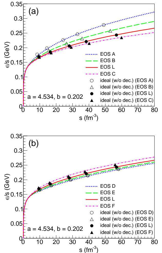
FIG. 2. (Color online) Energy over entropy versus entropy density for the equations of state shown in Fig. 1. Symbols correspond to Eq. (4) where \langle m_T \rangle and dN/dy are evaluated at T_f = 140 MeV in ideal hydrodynamics, before resonance decays.
