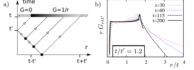
FIG. 4. a) Qualitative interpretation of the correlations in real-space in terms of a common virtual emitter in the past. G_{rtt'} vanishes in the dashed areas, where it is out of causal reach of virtual emitters. b) Rescaled two-times correlation function r G_{rtt'} as a function of r/t for t/t' = 1.2 . All data collapse on a step function as t increases, with finite size effects on scale \Lambda^{-1} .
