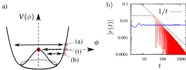
FIG. 1. a) Cartoon of the dynamical transition at the mean-field level. From top to bottom: quench above (a), at (t) and below (b) the dynamical transition. b) |r_t| for a quench within the unbroken symmetry phase (thick blue line) and at the dynamical transition (thin red line). In the second case, r_t decays faster than 1/t .
