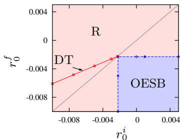
FIG. 5. Quench phase diagram: long time typical dynamics after a quench r_0^i \rightarrow r_0^f for \lambda = 1 . DT: Dynamical transition, OESB: Off-equilibrium symmetry breaking, R: Relaxation on large times to a non critical state. Error bars are smaller than item size. The exact position of transition lines depends on non-universal features, such as the interaction strength \lambda and the cutoff \Lambda .
