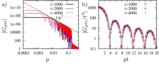
FIG. 3. a) Equal-time correlations |G_{ptt}| as a function of p for t = \{1000, 2000, 4000\} in a log-log scale. Notice the divergence of correlations below a cutoff scale p < \Lambda \simeq 0.2 . b) Rescaled equal-time correlations |G_{ptt}/t^2| as a function of pt for the same data, y-axis in log scale. All data collapse on the scaling law (7) drawn in black.
