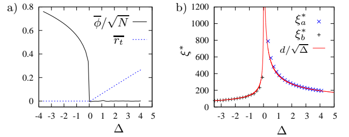
FIG. 2. a) Long time averages, \bar{\phi}/\sqrt{N} and \bar{r}_t , as a function of the relative distance to the critical point \Delta (in %). b) Critical length \xi^* versus \Delta the distance from the dynamical transition. Notice that despite the different definitions below and above the transition, \xi^* diverges as d/\sqrt{\Delta} on both sides of the transition, with d_a and d_b two different constants.
