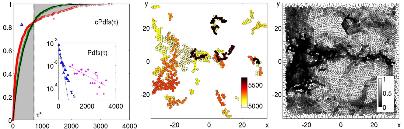
FIG. 4: Left: Cumulated probability distribution of the duration between spatially adjacent clusters (color online). Experimental data are in red circles while green squares stand for a set of equal cardinality generated from an exponential distribution with the same mean value. The black curve is the analytical version of this same distribution. The actual distribution and the exponential ones cross at the lag time \tau^* = 720 . Inset: Distribution of the lags below \tau^* (blue triangles) and above (magenta crosses). Middle: Spatial location of successive clusters of cage jumps. Colors correspond to the time at which clusters occur. Right: Spatial field of the two point correlation function Q_{p,t}(a^*, \tau^*) .
