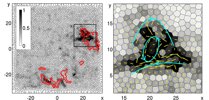
FIG. 3: Left: Clusters of cage jumps concentrate the highly non-affine domains : the distance to affinity parameter \Delta(t, \tau) (in levels of gray) is compared to the location of clusters of collective cage jumps (with red boundaries) ( \tau=30 ). Right: Zoom on a highly non-affine region (box on the left figure). The displacements of the particles, magnified by a factor 2, are in light grey (yellow online). For convenience, the main streams creating intense local shears are eye-guided.
