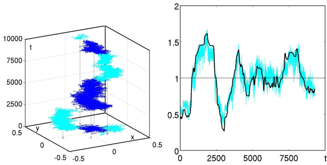
FIG. 1: Left: 3D visualization of the trajectory of a single particle. The color changes every time the algorithm detects a cage jump. Right: Comparison between the relative averaged relaxation Q_t(a^*, \tau^*) / \langle Q_t \rangle_t (in gray/cyan online) and the relative percentage P_t(\tau^*) / \langle P_t \rangle_t of particles that haven't jumped between t and t + \tau^* (in dark), \tau^* = 720 .
