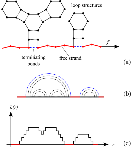
Fig. 1: (a) Illustration of the planar structure of RNA under tension, (b) rainbow diagram and (c) corresponding height relief.
