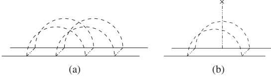
Fig. 2: Non-planar diagrams.
