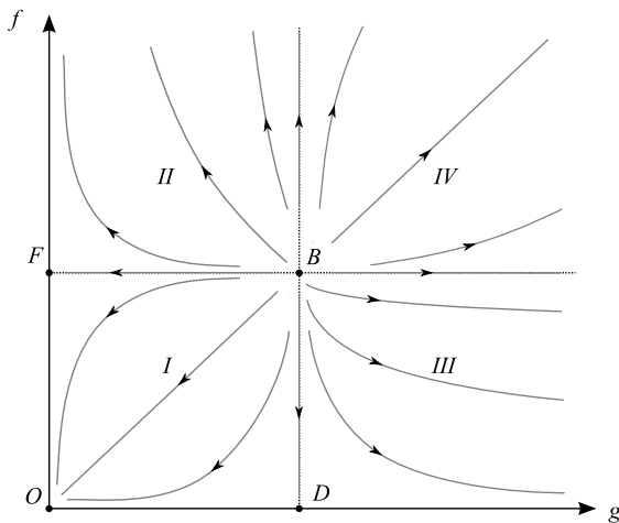
Fig. 3: Schematic view of renormalization group flow in the (g, f) -plane. The critical lines distinguish the molten phase (I), the denatured homopolymer phase (II), a glass phase (III). A new phase (IV) corresponds to RNA strands with isolated frozen structures separated by free parts.
