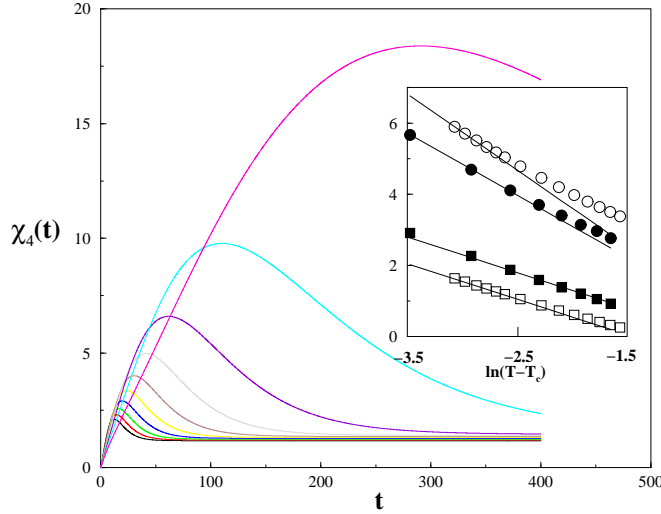
Fig. 2 – Four-point susceptibility \chi_4(\tau) in the mean-field p = 3 spin-glass, obtained by integrating the dynamical equations obtained in [11], for various temperatures T > T_c ( T_c = 0.612 ). The inset shows, in semi-log, the position t^* (black circles) and the height \chi_4(t^*) (black squares) of the peak as a function of T - T_c , and the plain lines are power-laws with exponents -1 and -(1+a)/2a = -1.76 , corresponding to the ‘naive’ argument discussed in the text. We confirmed these results by also solving numerically the mixed p = 3 + 6 case, for which a = 0.345 and b = 0.717 (open symbols). These last curves have been shifted for clarity.
