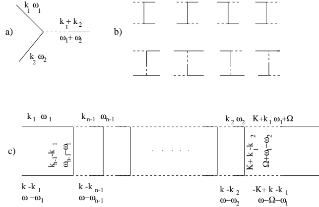
Fig. 1 – Basic vertex of the MCT (a), and a ladder diagram that contribute to the divergence of the four-point susceptibility (c). Other ladders can be obtained by combining the eight elementary blocks shown in (b). The full lines represent correlation functions, whereas the mixed dashed-full lines are response functions.
